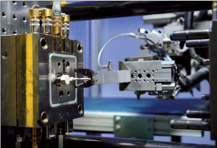
Fig. 4 Extraction of an injection molded part
